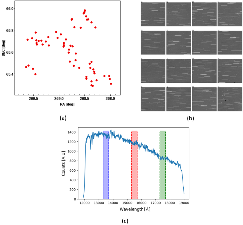
Figure 1. Simulation of the self-calibration procedure (Passalacqua, 2022). a) shows the optimize sequence of pointings; b) shows the simulation of the images detected by NISP detectors; c) shows the extracted 1D counts from the raw images. The regions in different colors represent the integration range for each selected wavelength.
